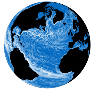
Ocean simulation performed with the NEMO code.
